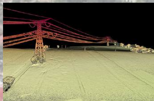
Cross Section of Acquired Point Cloud from Microdrones mdLIDAR-1000
